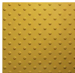
Yellow tactile warning Surface (Diagonal alignment number 2) Product Code: 4U0568 Size: 400 X 400 X 8 mm Material: TPU
