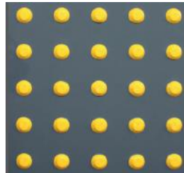
Dual Color Gray - Yellow Tactile Warning Surface Product Code: 4U0552M Size: 300 X 300 X 8 mm Material: TPU
