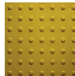
Yellow tactile warning surface (Parallel alignment) Product Code: 4U0554$ Size: 400 X 400 X 8 mm Material: TPU
