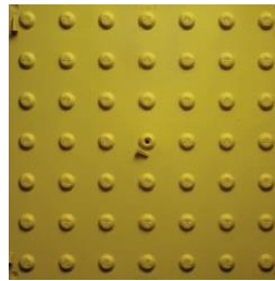
CTP Tactile Warning Surface (With Screw) Product Code: 4U0589 Size: 400 X 400 X 8 mm Material: CTP
