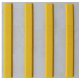
Dual Color Transparent - Yellow Tactile Directional Surface Product Code: 4U0551S Size: 300 X 300 X 8 mm Material: TPU
