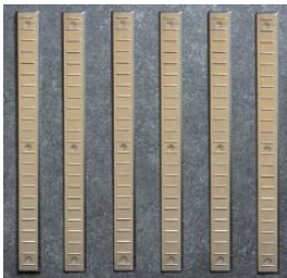
Stainless Steel Tactile Directional Surface Product Code: 4U0571 Size: 400 X 400 X 8 mm Material: 304 stainless steel
