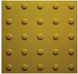
Yellow Tactile Warning Surface Product Code: 4U0552 Size: 300 X 300 X 8 mm Material: TPU
