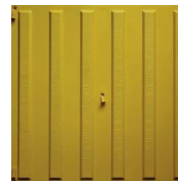
CTP Tactile Directional Surface (With Screw) Product Code: 4U0588 Size: 400 X 400 X 8 mm Material: CPU
